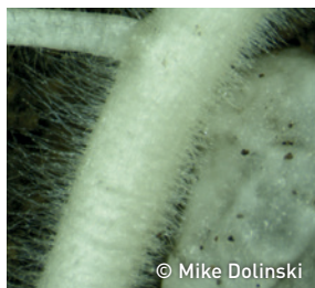
Pea root interacting with Polyhalite.
