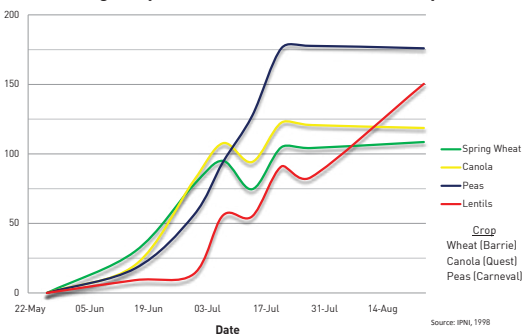
Nitrogen Uptake & Demand for Selected Crops
