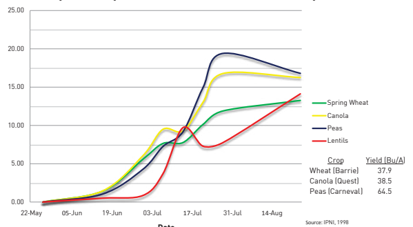
Phosphorus Uptake & Demand for Selected Crops
